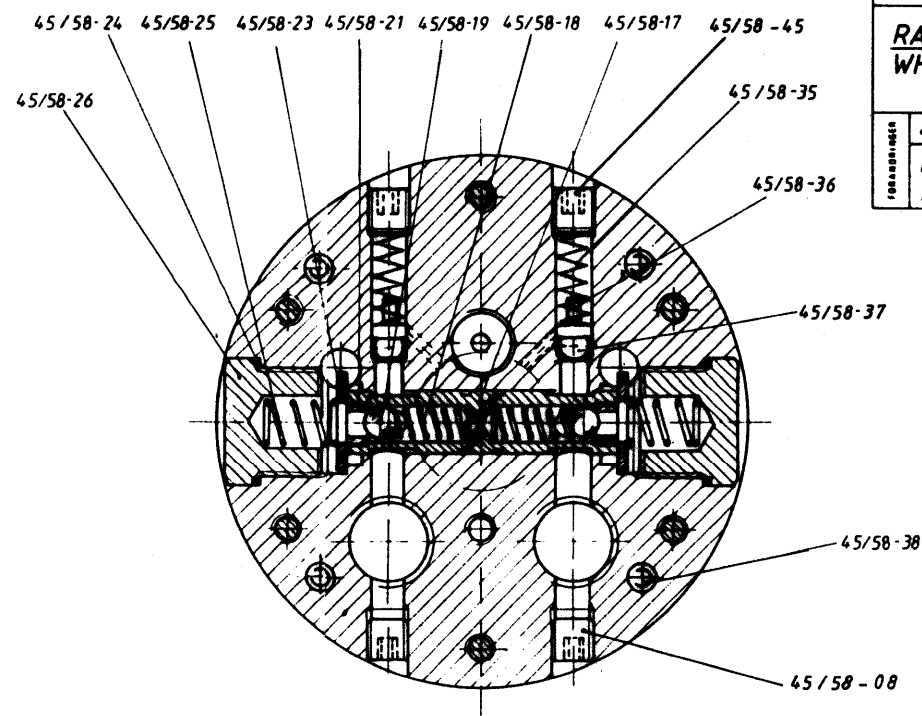
SNITT SECTION B-B
