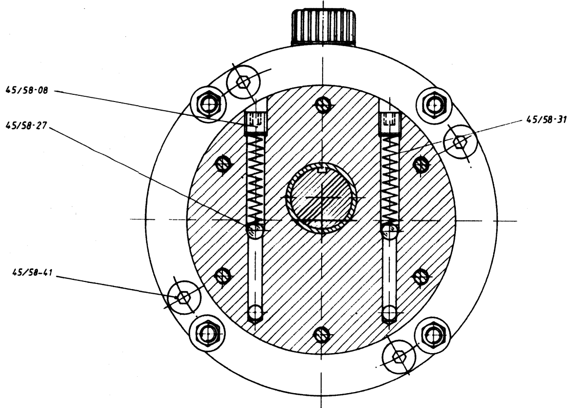
SNITT SECTION C-C
